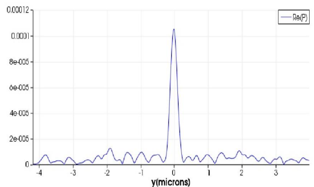
Fig. 5A. Simulation for NOR Gate [11]
