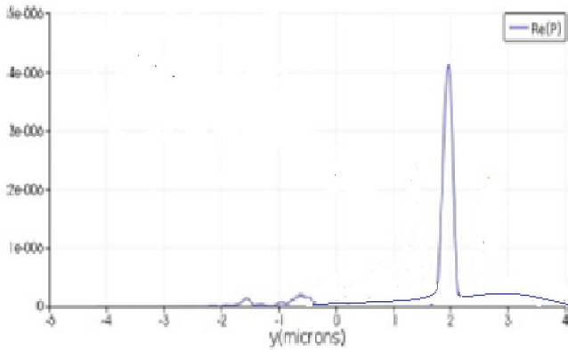
Fig. 3A. Simulation for OR Gate [01]
