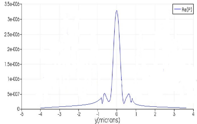
Fig. 4B. Simulation for NOT Gate [01]
