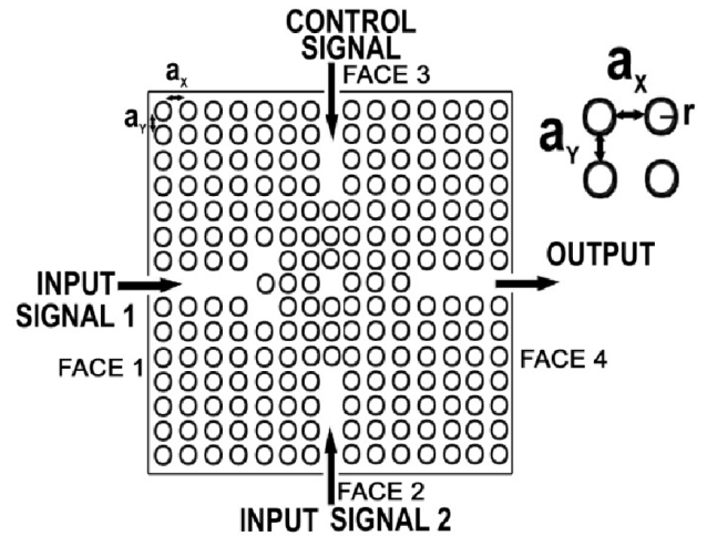
Fig 1. Proposed 2D PCS for Logic Gate
