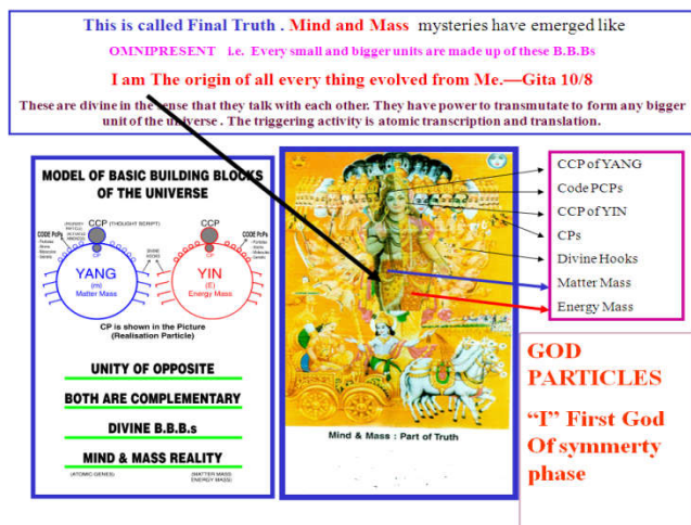
Fig. 1. Divine Mechanics Unit – CCP, CP and information s – Code PCs with B-Bit – Mass
