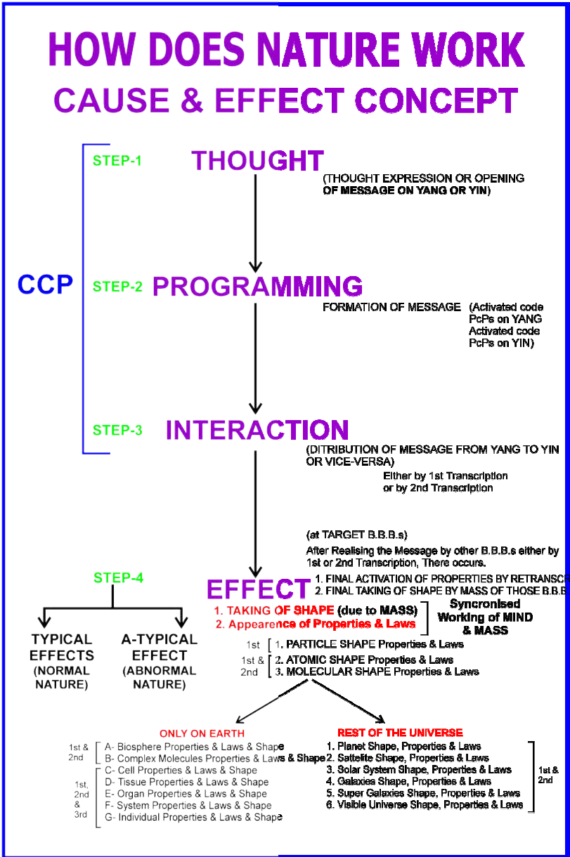
Fig. 6. Divine Mechanics – How Does Nature work ?
