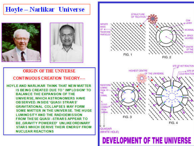
Fig. 9. Development of the Universe
