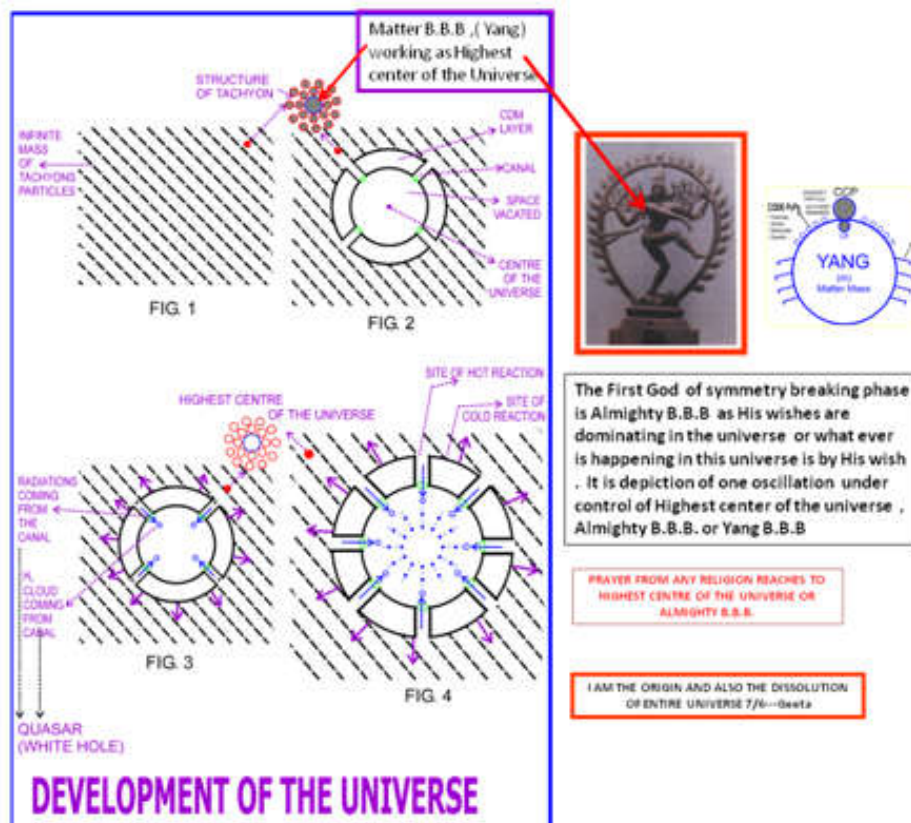
Figure 9.1. Hoyle Narlikar Universe
